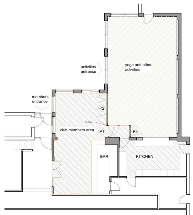
NEW REMOVABLE PARTITIONS FULLY CLOSED- MORNING AND AFTERNOON USE
