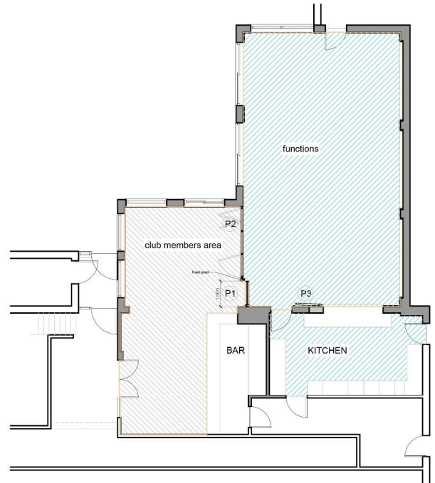
NEW REMOVABLE PARTITIONS PARTIALLY OPEN- OCCASIONAL EVENING USE DIAGRAM
